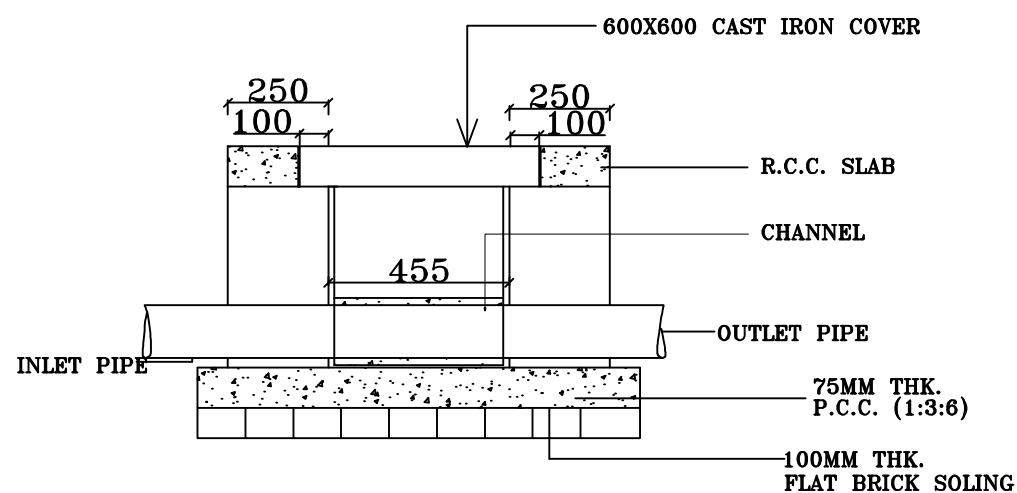
DETAIL OF INSPECTION CHAMBER
